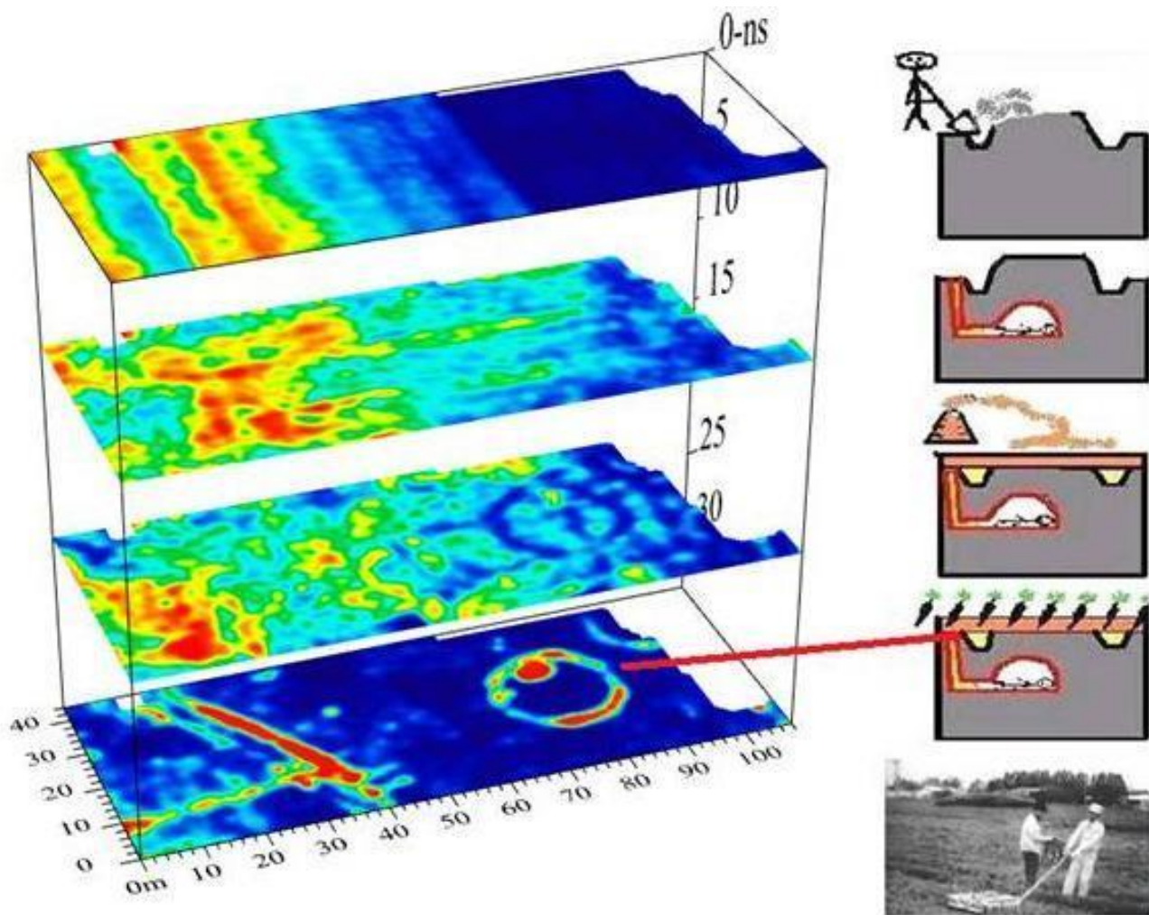
Figure 7. A set of horizontal section (plan) images from the GPR survey of a buried grave with surrounding ditch. A series of pictures illustrate the development of the soil after the grave's construction (on the right, top to bottom). (Image from the website of GPR-SLICE software at http://www.gpr-survey.com/gprslice2.html where further images and videos explaining the use of 3D data can be found).
