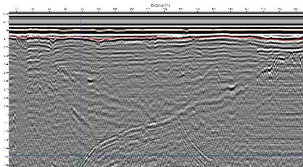
Figure 6. Radargram profile (depth section) from a GPR investigation showing a series of probable older road surfaces underneath the current surface level, as well as possible stratigraphic boundaries deeper down. For archaeological applications it is preferable to combine such transects with a series of horizontal slices (plans) to help understand the changes that have occurred over time at different depths. Archaeological GPR exploration is most usefully undertaken in 3D, using software such as GPR-SLICE ( http://www.gpr-survey.com/ ), ApSoft 2.0 ( http://archpro.lbg.ac.at/apsoft-20 ) (see Figure 7). Image created by Ramböll RST and provided by Trafikverket.
