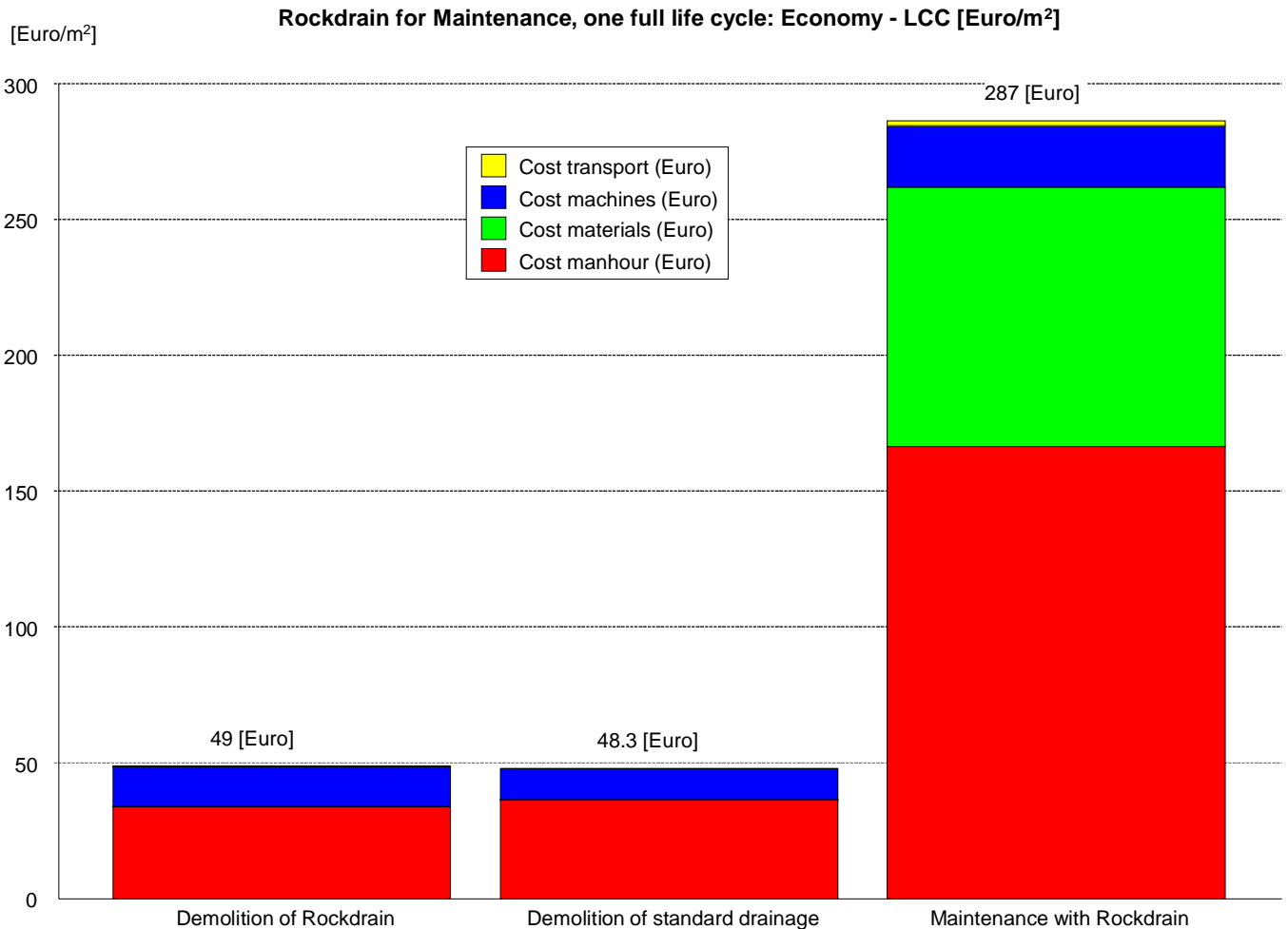
Figure 14 Results from the LCA model of Rockdrain as maintenance measure showing the economy as LCC. The results show the maintenance procedure with Rockdrain and the preceding demolition of either a conventional standard drainage or a Rockdrain drainage. This figure shows the results for the entire life cycle of Rockdrain (120 years) and the entire life cycle of the standard drainage (60 years) respectively. Thus, this figure shows one life cycle of both Rockdrain and standard drainage.
