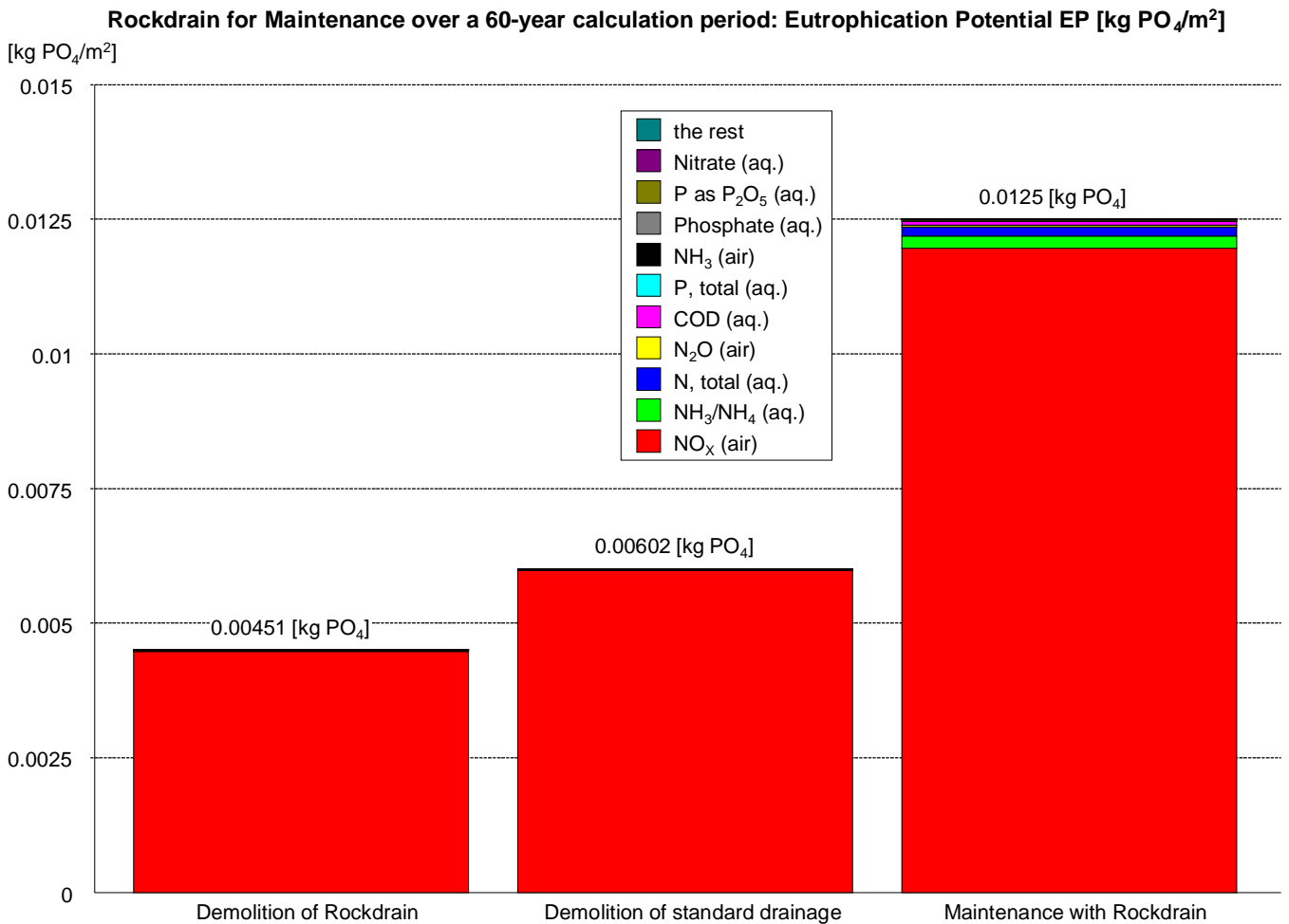
Figure 7 Results from the LCA model of Rockdrain as maintenance measure showing the eutrophication potential (EP). The results show the maintenance procedure with Rockdrain and the preceding demolition of either a conventional standard drainage or a Rockdrain drainage. This figure shows the results for a calculation period of 60 years with a lifespan for Rockdrain of 120 years and for conventional drainage of 60 years.
