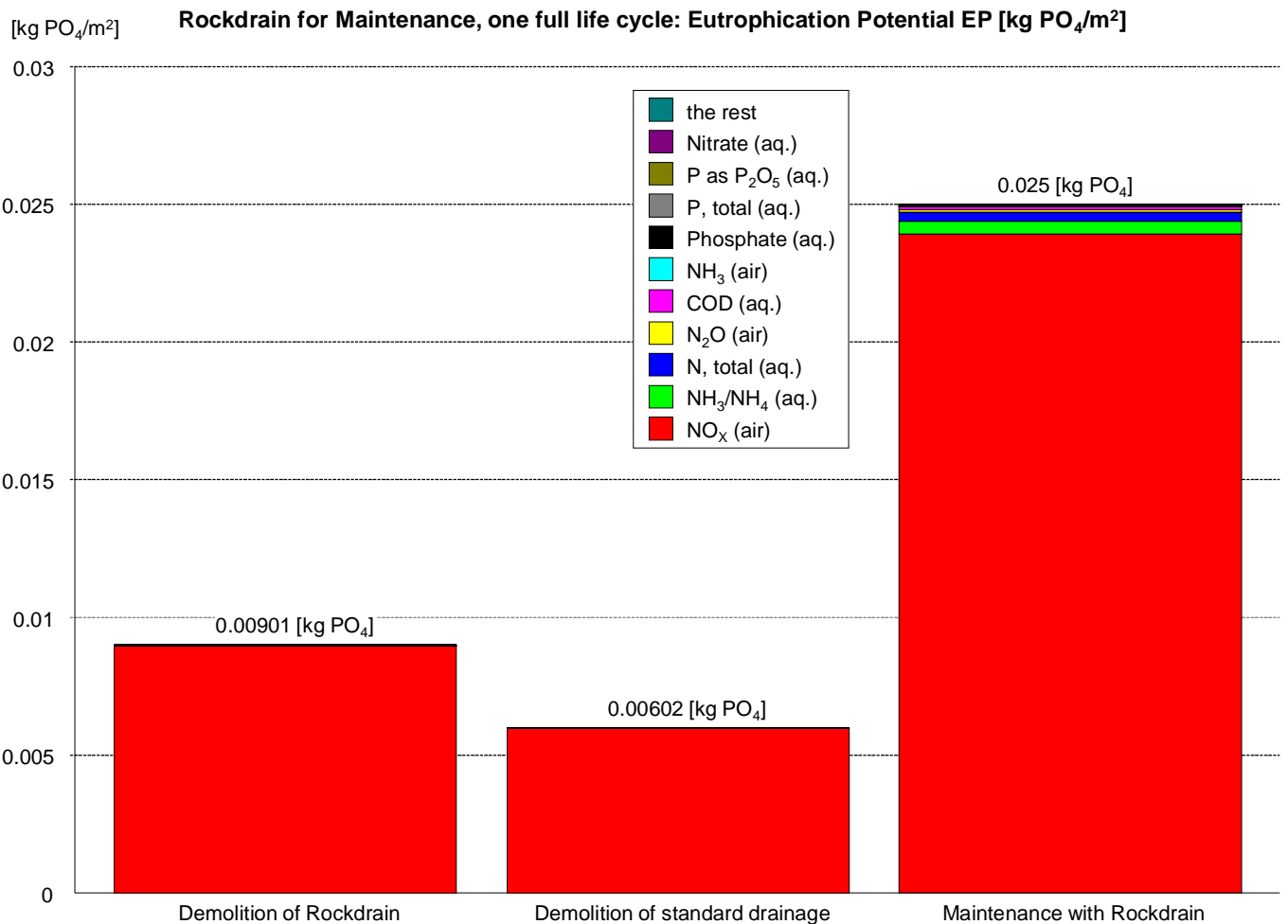
Figure 8 Results from the LCA model of Rockdrain as maintenance measure showing the eutrophication potential (EP). The results show the maintenance procedure with Rockdrain and the preceding demolition of either a conventional standard drainage or a Rockdrain drainage. This figure shows the results for the entire life cycle of Rockdrain (120 years) and the entire life cycle of the standard drainage (60 years) respectively. Thus, this figure shows one life cycle of both Rockdrain and standard drainage.
