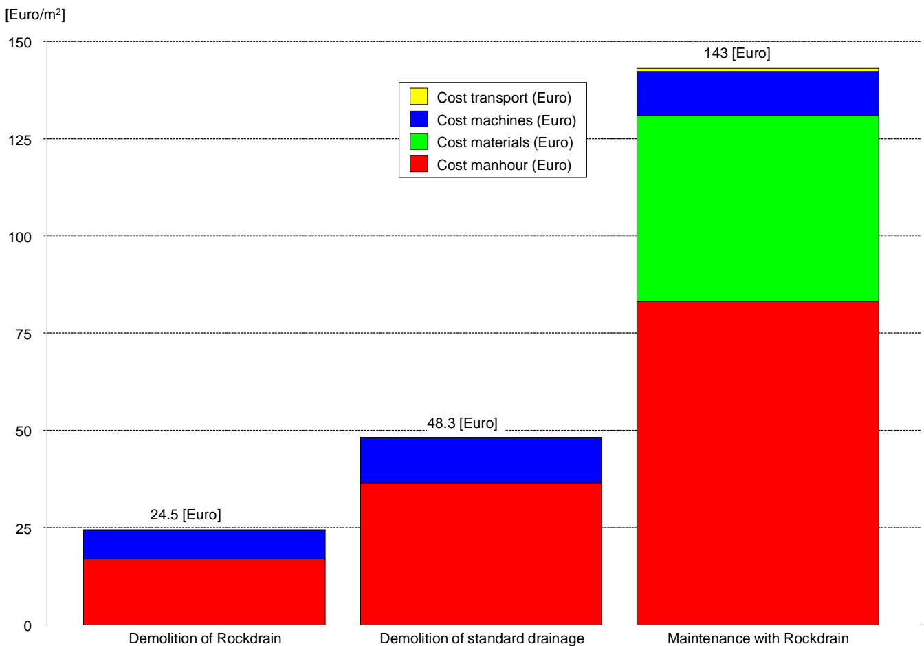
Rockdrain for Maintenance over a 60-year calculation period : Economy - LCC [Euro/m 2 ]
