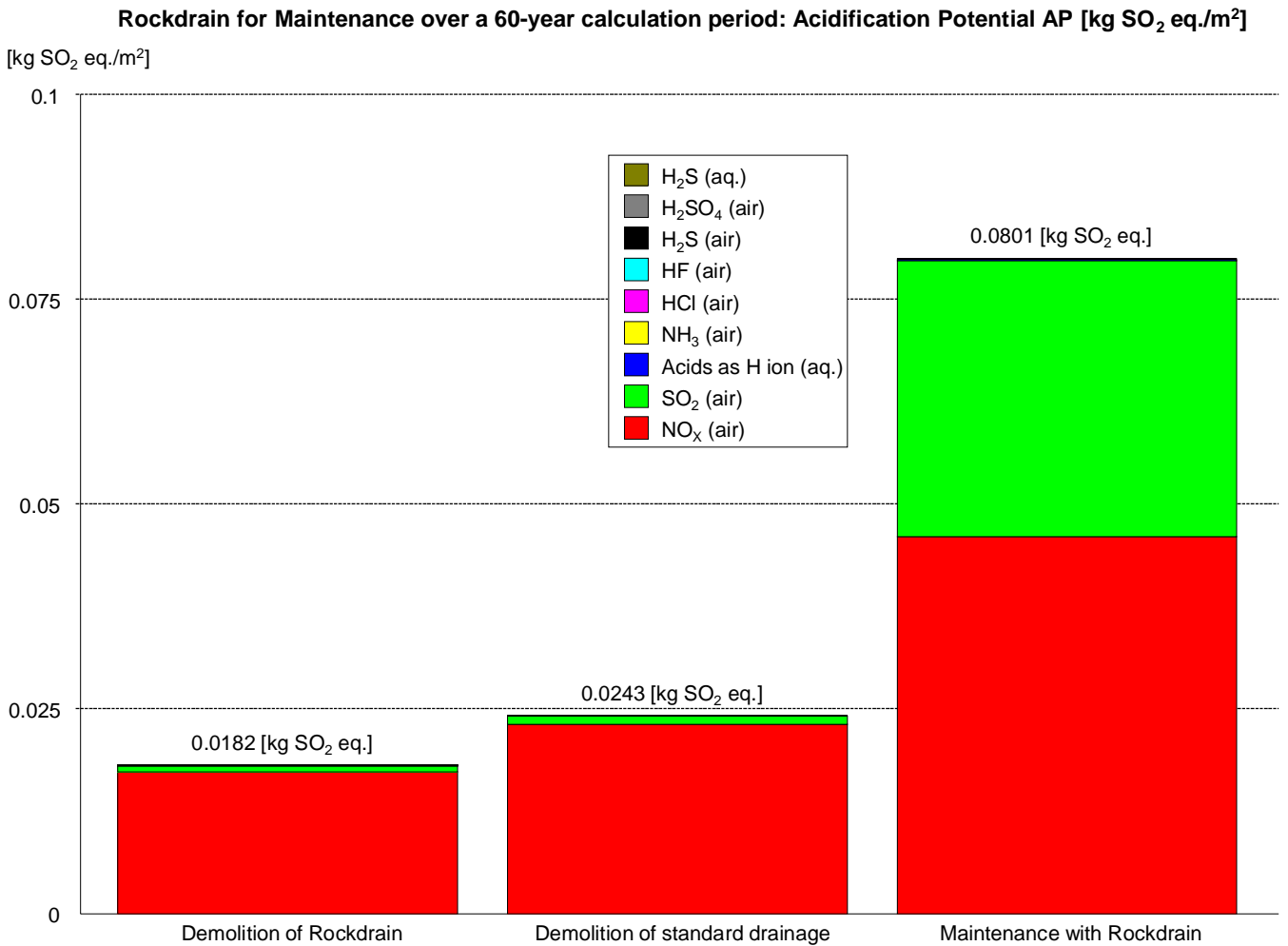
Figure 5 Results from the LCA model of Rockdrain as maintenance measure showing the acidification potential (AP). The results show the maintenance procedure with Rockdrain and the preceding demolition of either a conventional standard drainage or a Rockdrain drainage. This figure shows the results for a calculation period of 60 years with a lifespan for Rockdrain of 120 years and for conventional drainage of 60 years.
