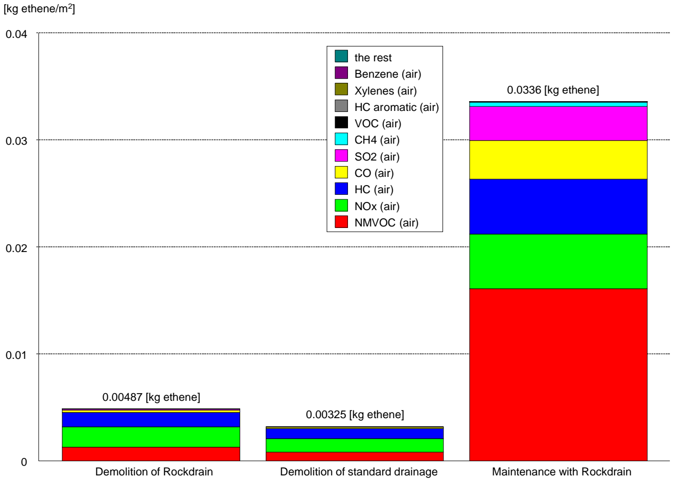
Figure 10 Results from the LCA model of Rockdrain as maintenance measure showing the photochemical ozone creation potentials (POCP). The results show the maintenance procedure with Rockdrain and the preceding demolition of either a conventional standard drainage or a Rockdrain drainage. This figure shows the results for the entire life cycle of Rockdrain (120 years) and the entire life cycle of the standard drainage (60 years) respectively. Thus, this figure shows one life cycle of both Rockdrain and standard drainage.
