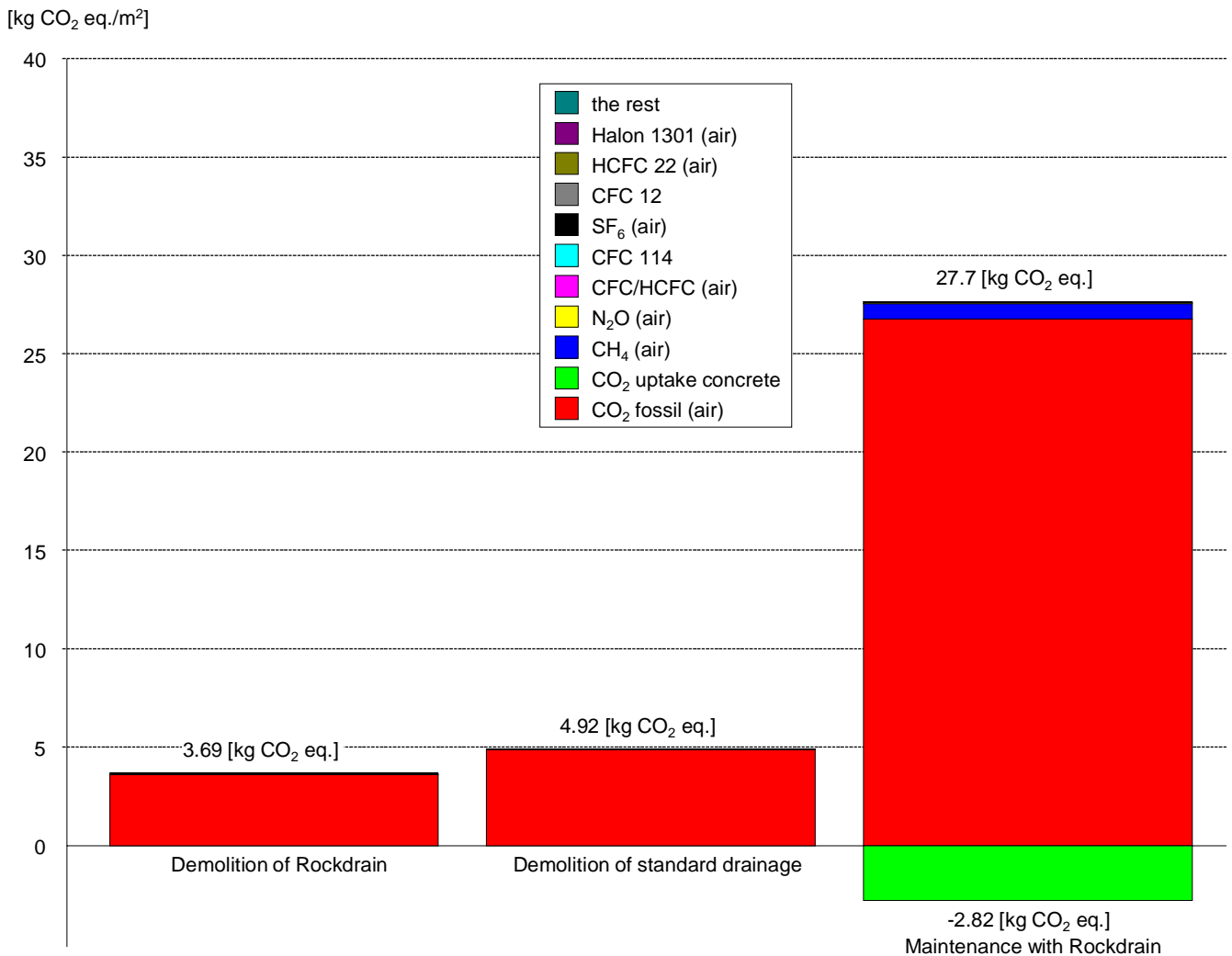
Rockdrain for Maintenance over a 60-year calculation period: Global warming GWP 100 [kg CO 2 eq./m 2 ]
