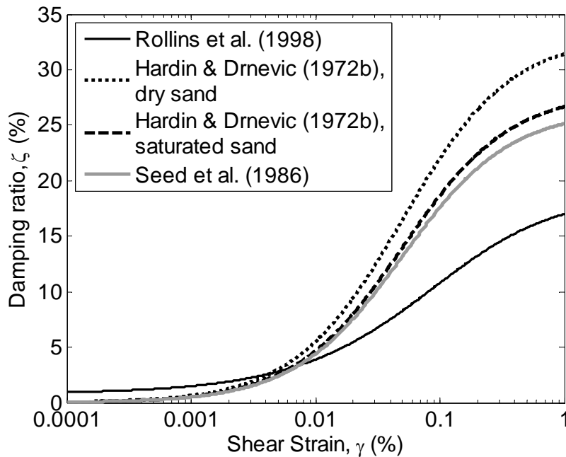
Figure 16. Comparison of damping ratio by different models.
