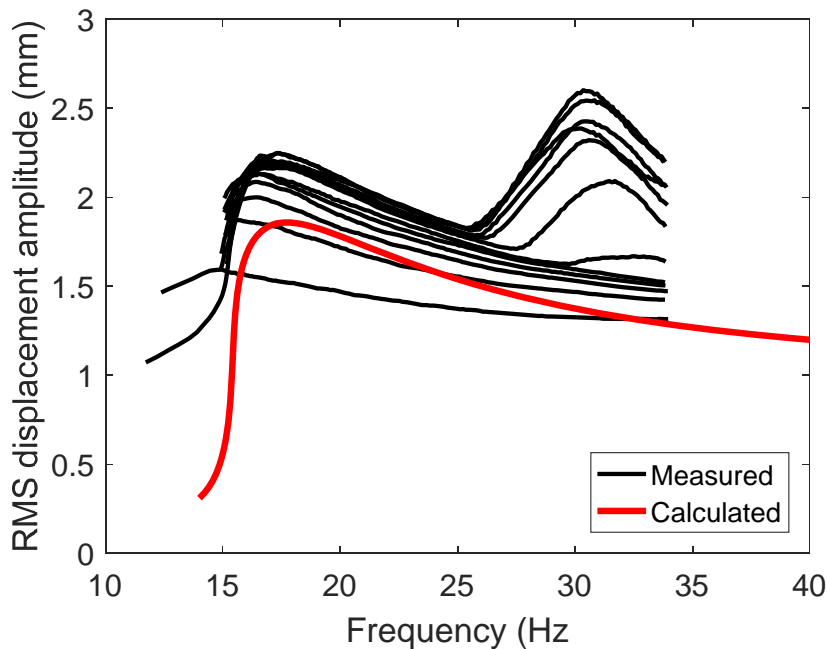
Figure 17. Measured and preliminary calculated dynamic displacement of the drum in the full-scale tests.
