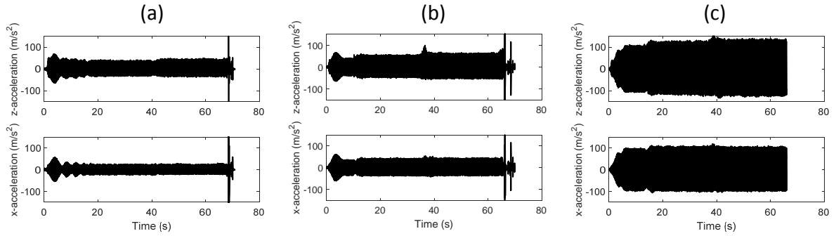
Figure 5. Examples of vertical and horizontal acceleration on the drum, (a) below resonance, (b) at resonance and (c) above resonance.
