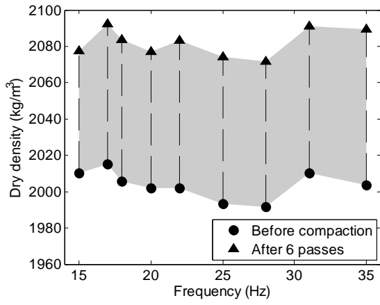
Figure 10. Average density before and after compaction.
