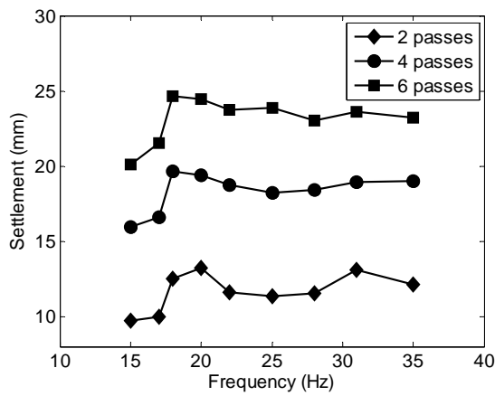
Figure 8. Average settlement.
