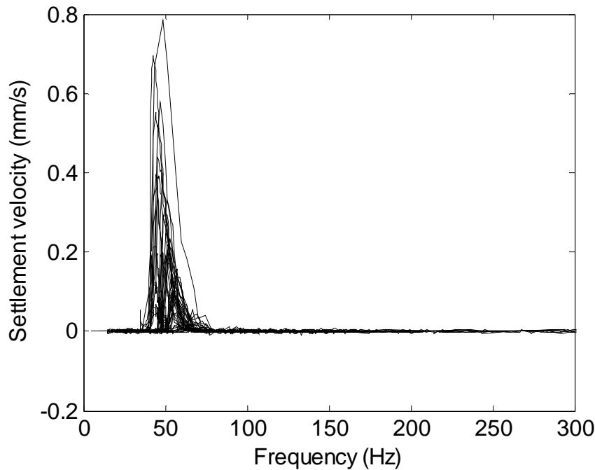
Figure 18. Settlement velocity in tests using electro-dynamic oscillator. Modified after Paper I.
