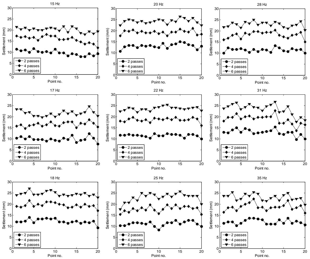
Figure 7. Settlement along the test surface for all frequencies. Each data point represents the average of three measuring points.
