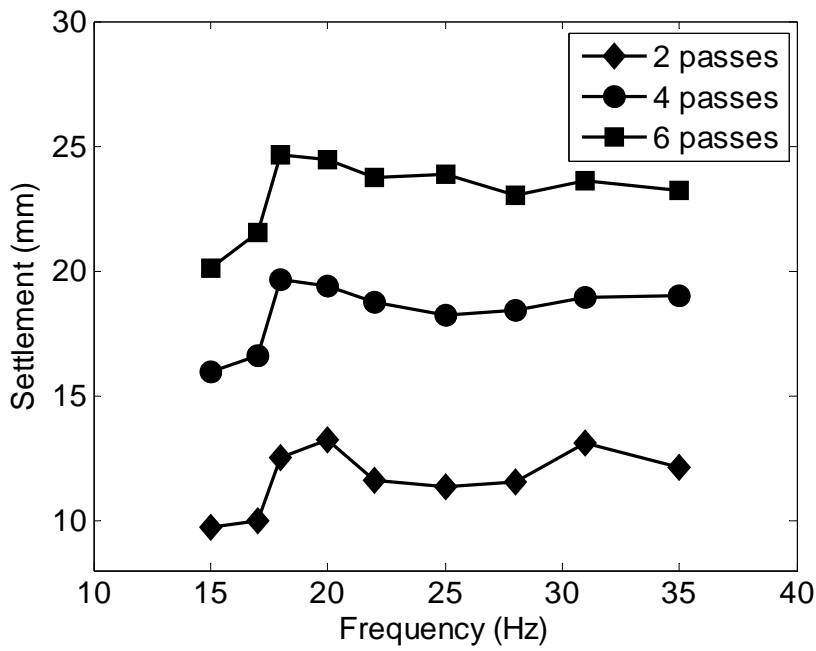
Figure 20. Frequency-dependent settlement in full-scale tests.
