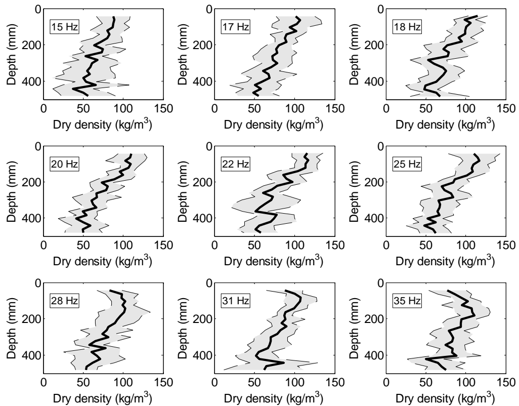
Figure 9. Density increase from six passes for each frequency.
