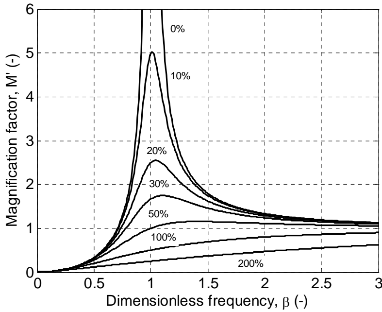
Figure 12. Dynamic magnification factor for rotating mass oscillators and different damping ratios.
