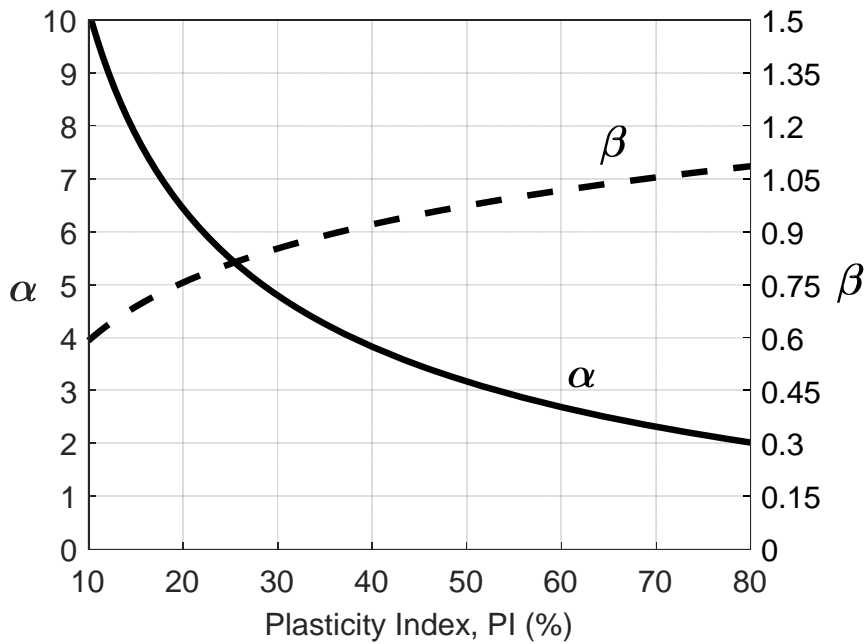
Figure 14. Variation of \alpha and \beta with PI (after Massarsch 2004).
