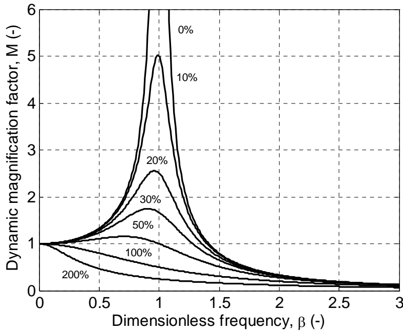
Figure 11. Dynamic magnification factor for constant force and different damping ratios.
