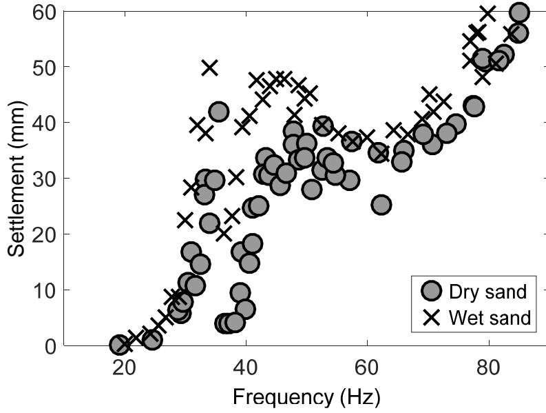
Figure 19. Total settlement in tests using rotating mass oscillators. From Paper V.
