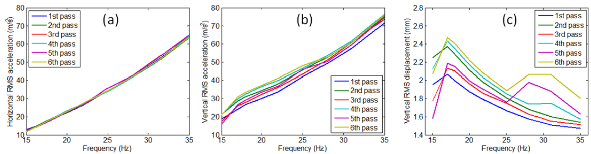
Figure 6. Calculated RMS values, as a function of frequency, of (a) horizontal acceleration, (b) vertical acceleration and (c) vertical displacement.
