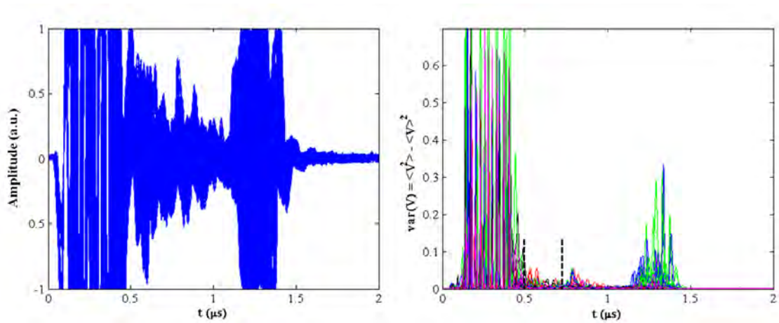
Figure 5.3: CFRP sample set 1, Set-up A: Left side: All signals from all damage states, Right side: All variances from all damage states. Time window is marked.
