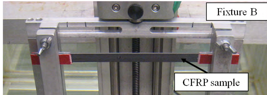
Figure B.2: One of the CFRP samples.
