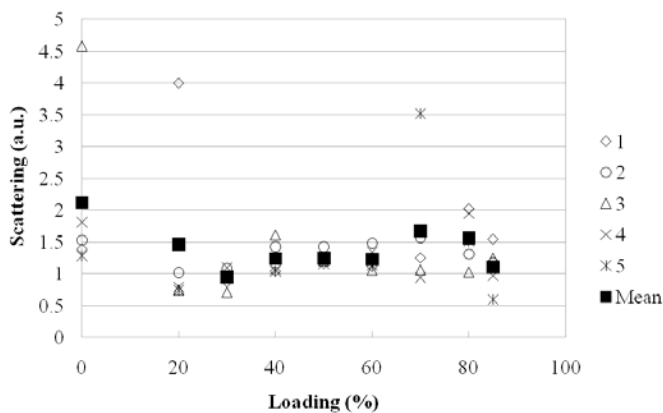
Figure 4.12: Set-up E: Integration of time window, 6.3 - 9 \mu s.
