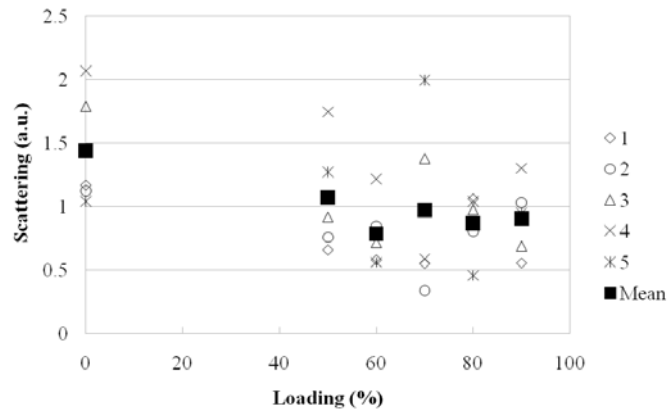
Figure 4.14: Set-up A: Integration of time window, 0.5 - 0.75 \mu\text{s} .
