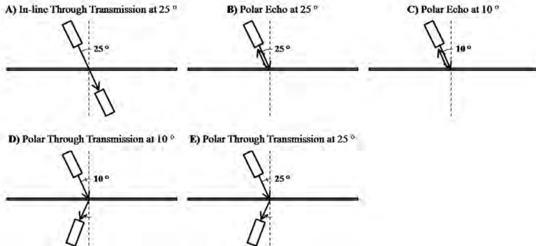
Figure 3.24: The five different experimental set-ups called A to E.
