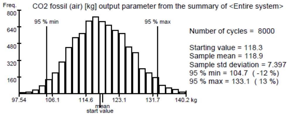
Figure 38 Results from a sensitivity analysis of CO 2 fossil emissions from the model of the conventional drainage system.
